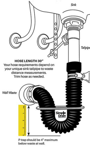
STEP 4 THREAD TO WASTE Fits standard 1.5" male threaded connection.
